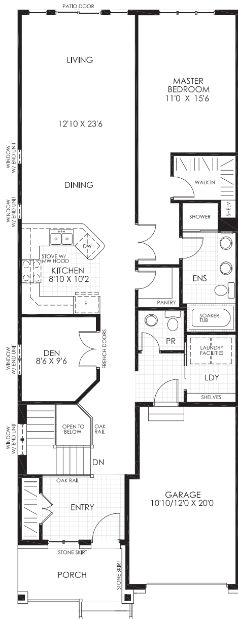
GROUND FLOOR
